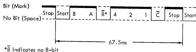
Figure 5. Bit Configuration of a "G" Character (Serialized)
