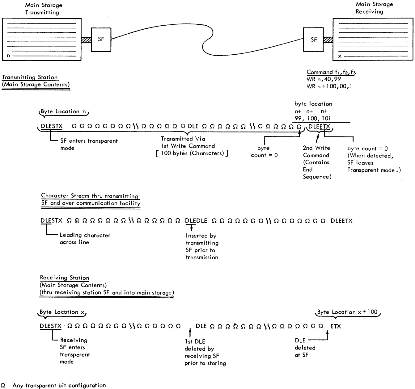
Figure 15. Transparent Operation
