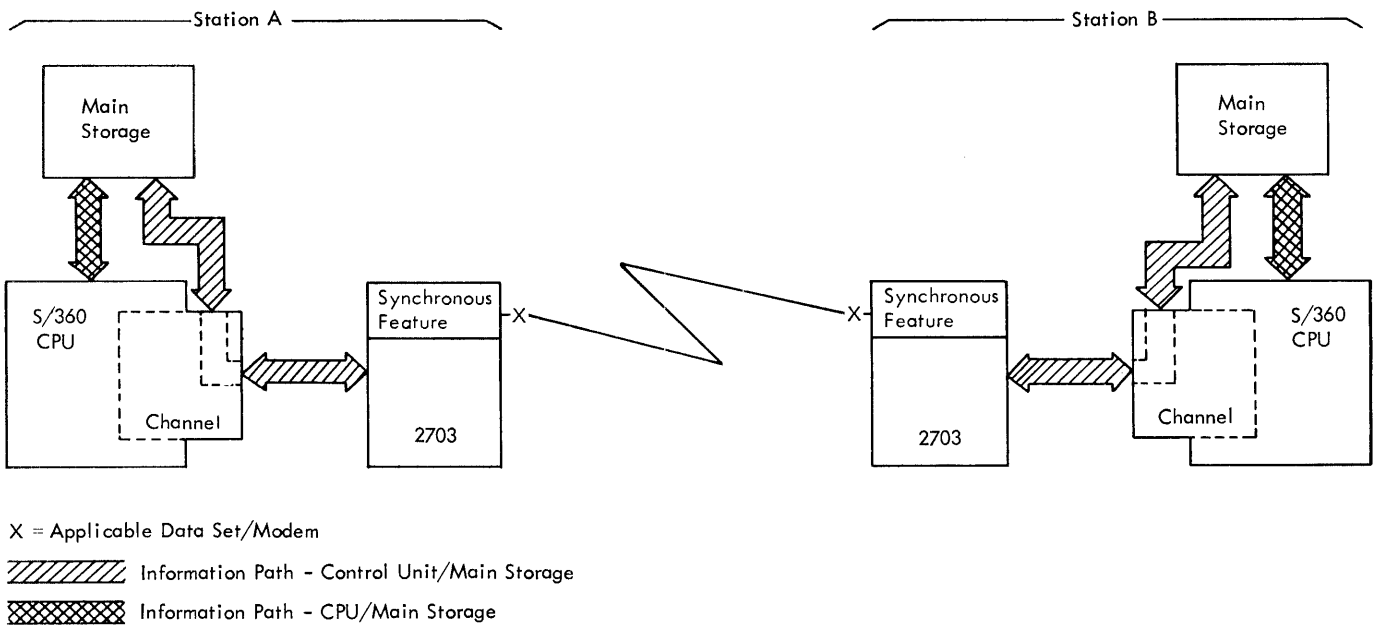
Figure 11. Operation of Two System/360 Computers over a Communications Line
