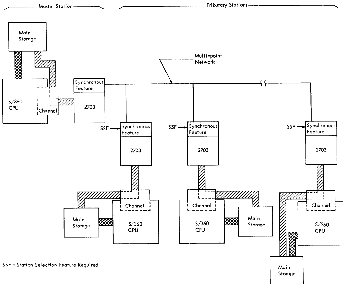
Figure 14. Multipoint Configuration
