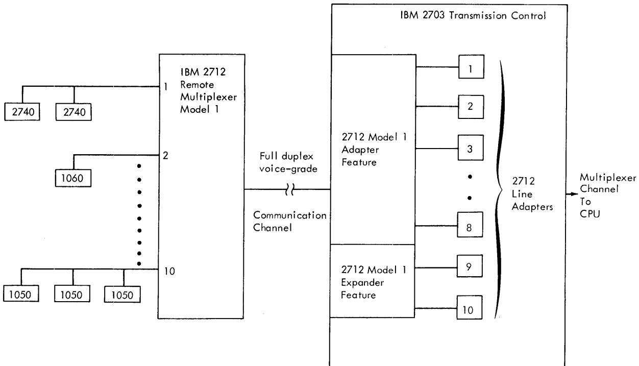
Figure 9. Typical 2712 Configuration
