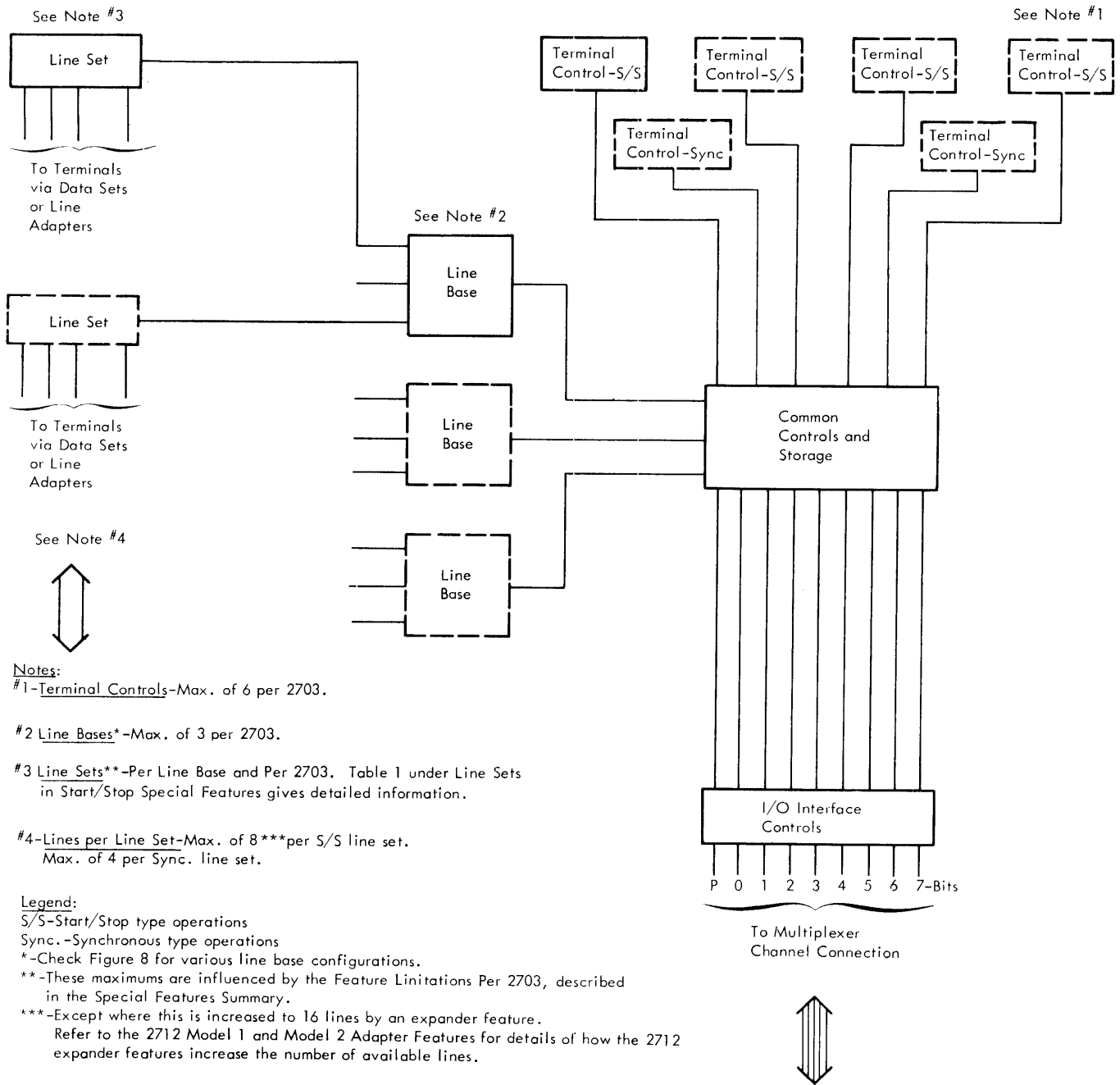
Figure 3. 2703-Internal Organization
