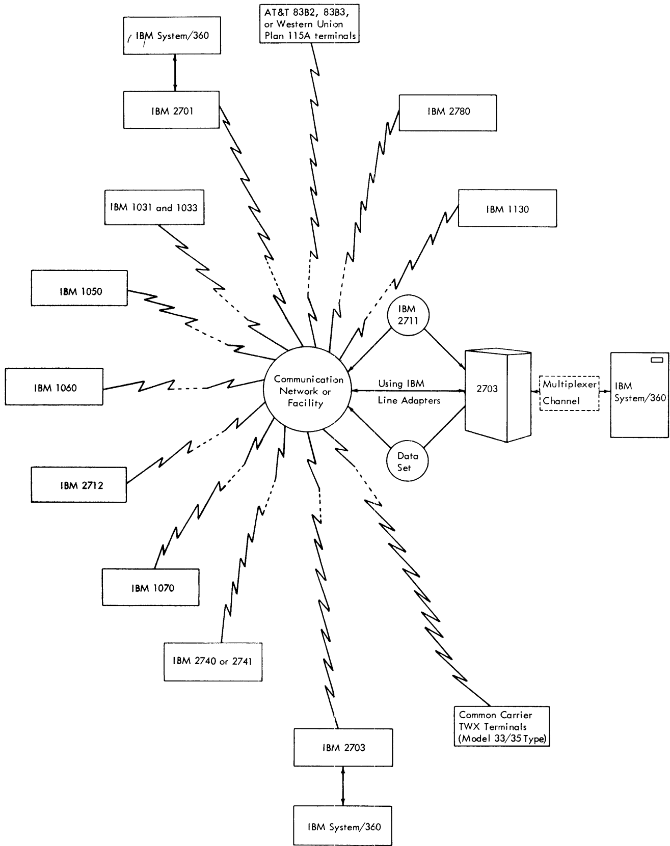
Figure 2. Data Communication Units Attachable to the 2703
